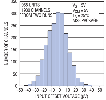
Typical Distribution of Over-The-Top Input Offset Voltage
