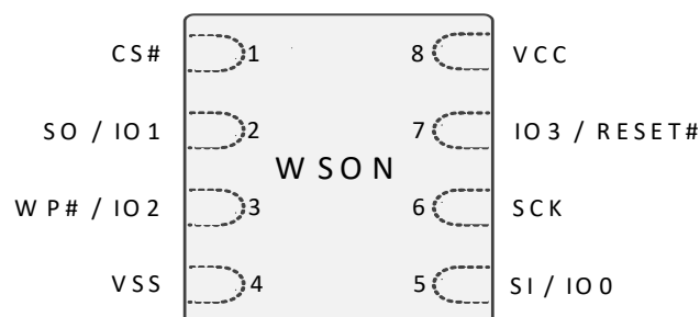
Figure 4. 8-Connector Package (WSON 5 x 6), Top View [3]
