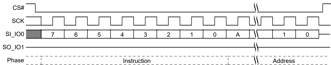
Figure 84. Block Erase (BE D8h or 4BE DCh) Command Sequence [48]
