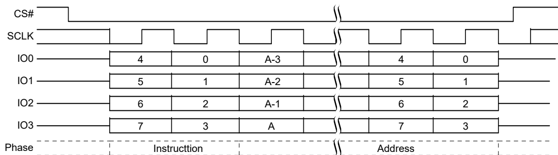
Figure 81. Sector Erase (SE 20h or 4SE 21h) QPI Mode Command Sequence [45]
