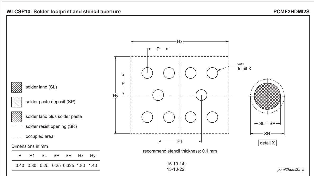
Fig 23. Soldering footprint WLCSP10 (PCMF2HDMI2S)
