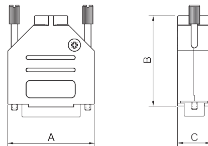
D-Sub-Hood
