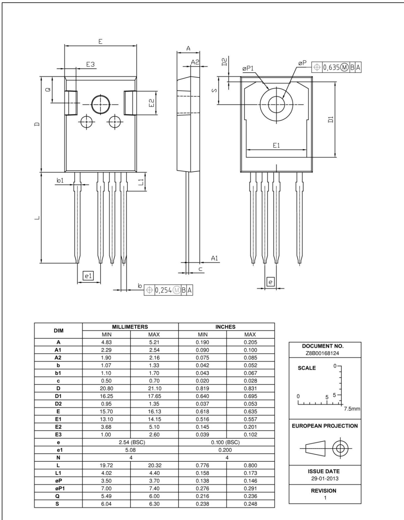
Figure 22 Package drawing
