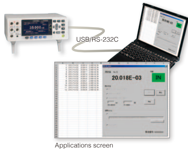
Applications screen
