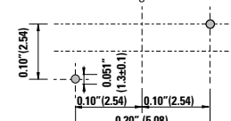
Circuit Board Mounting Detail
