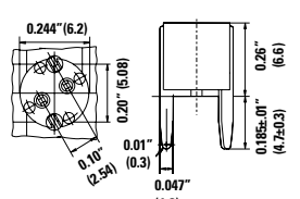
55600000001 Black / Vertical Mount Devices
