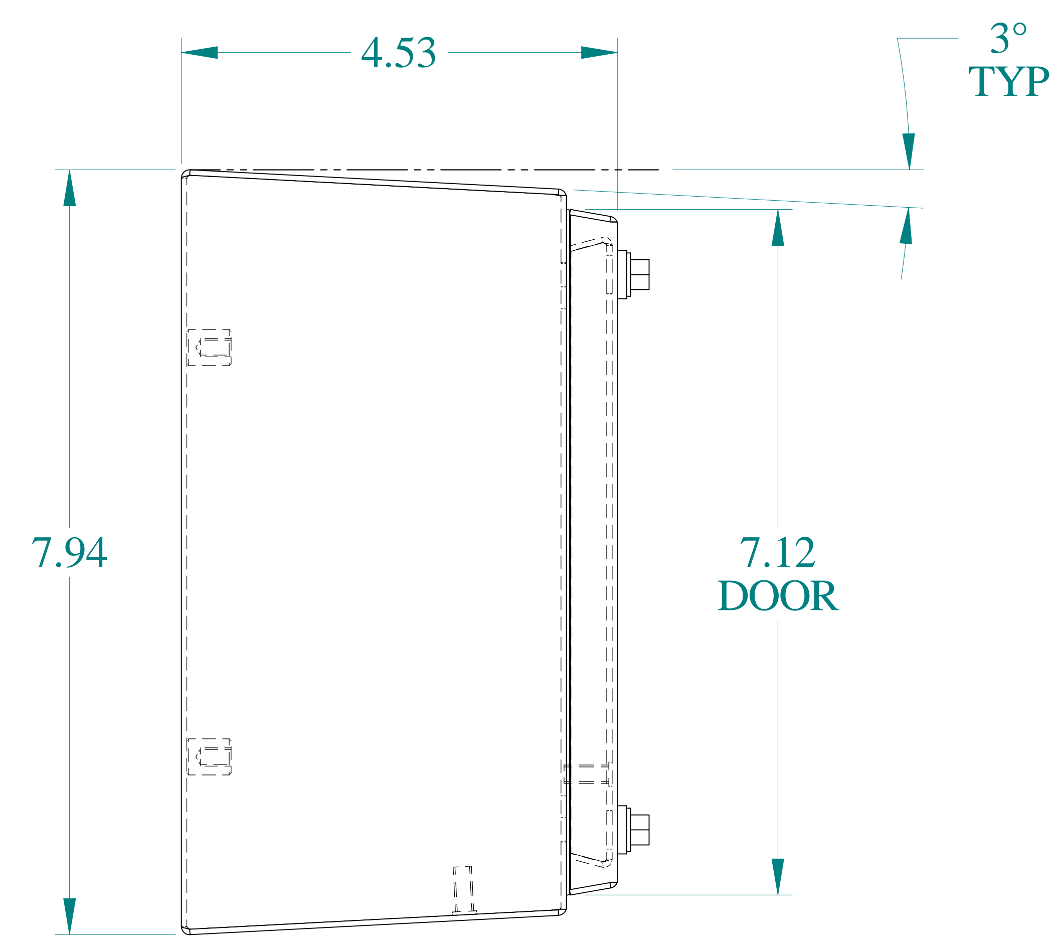
SIDE VIEW
