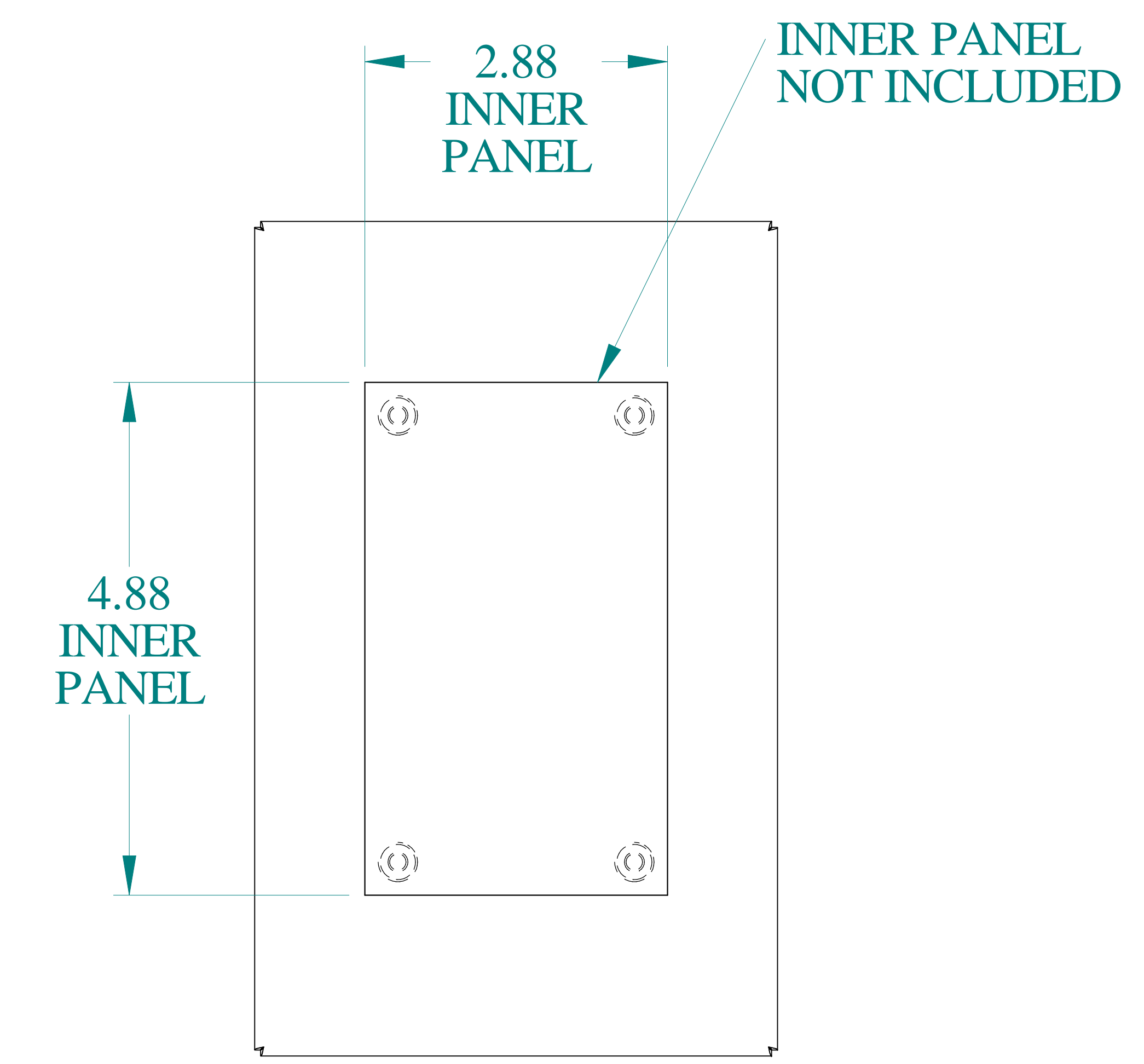
BACK VIEW
