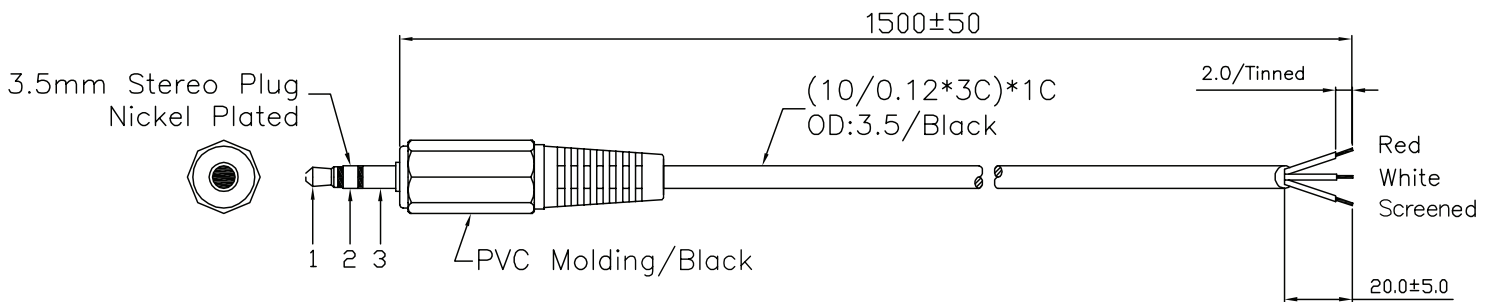
Soldered Drawing: 3.5mm Stereo Plug
