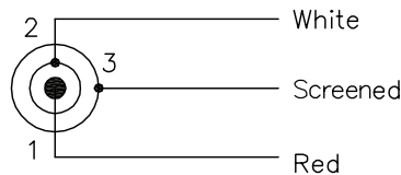
Soldered Drawing: 3.5mm Stereo Plug
