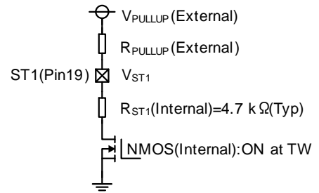
Figure 71. ST1 Pin Circuit for TW
