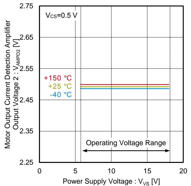
Figure 41. Motor Output Current Detection Amplifier Output Voltage 2 vs Power Supply Voltage
