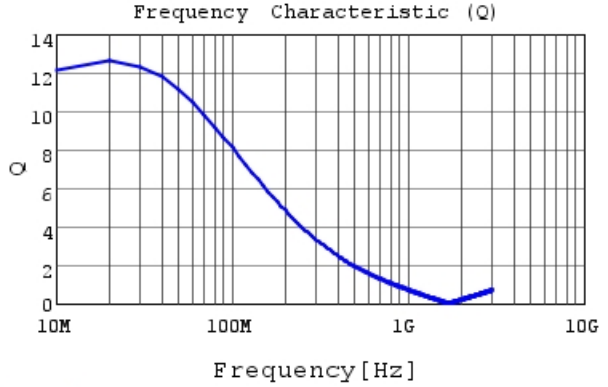
LQW18CNR21J0H Q
