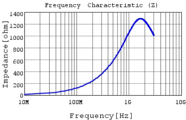
LQW18CNR21J0H |Z|
