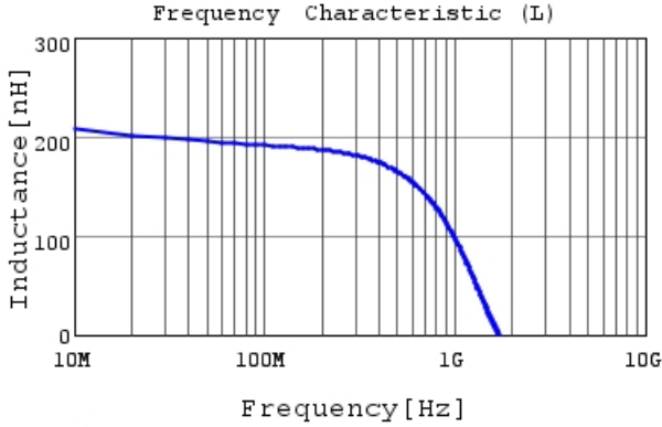
LQW18CNR21J0H L
