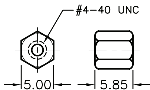
Nut (4pcs)
