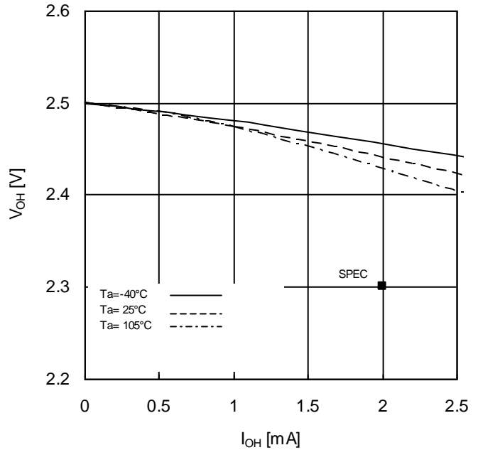
Figure 8. Output High Voltage vs Output Current (V<sub>CC</sub>=2.5V)
