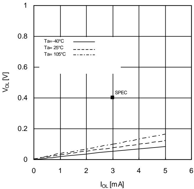
Figure 7 Output Low Voltage vs Output Current (V<sub>CC</sub>=2.5V)
