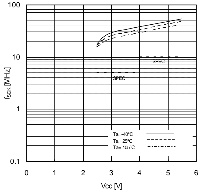
Figure 14. SCK frequency vs Supply Voltage
