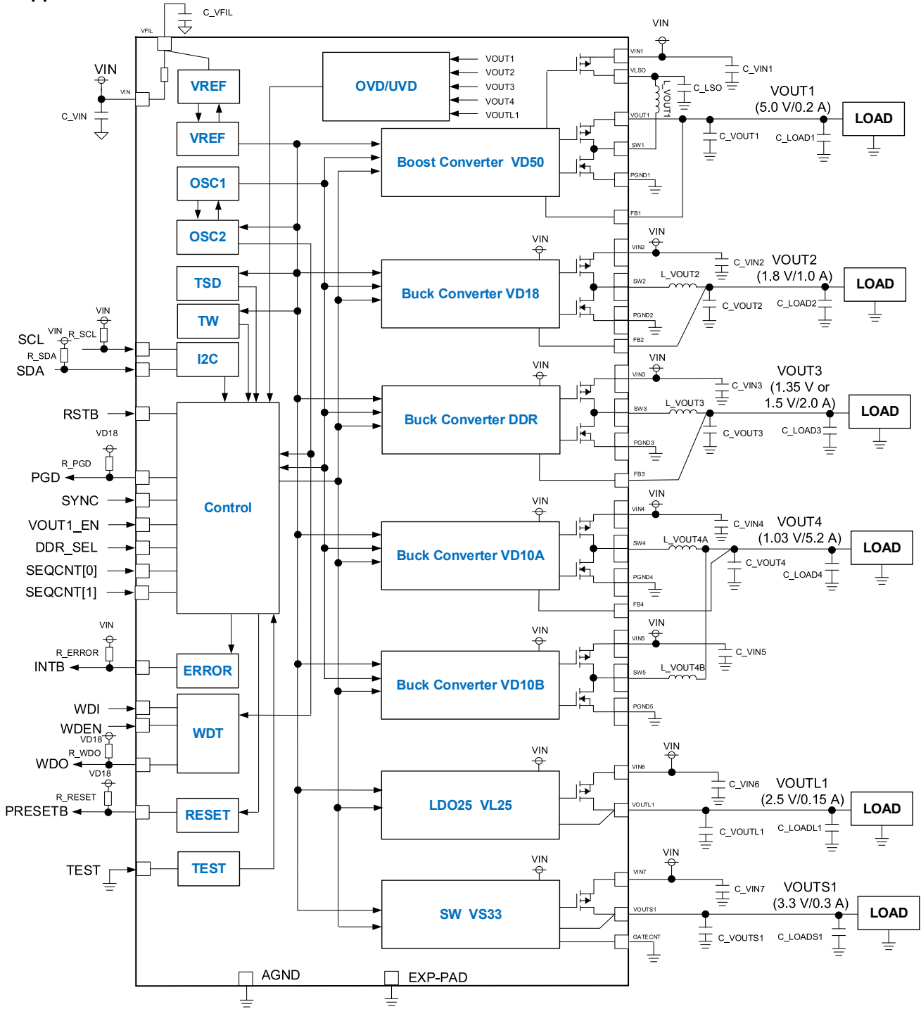
Figure 2. Application Circuit
