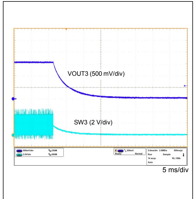
Figure 67. VOUT3 Power OFF Waveform (VOUT3 = 1.5 V Setting)
