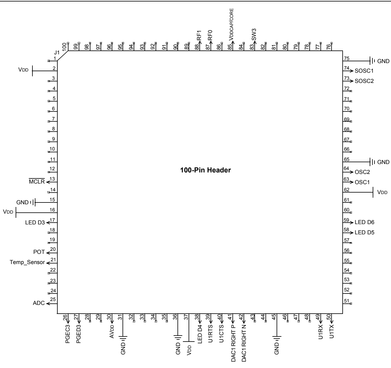
FIGURE 1: 100-PIN HEADER SCHEMATIC
