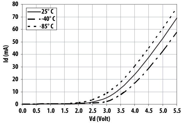
Figure 41. Current vs Voltage and Temperature
