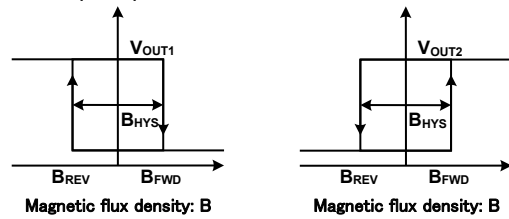
Figure 4. Output operation
