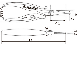
Part No. 106-07
