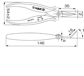
Part No. 106-08
