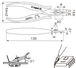
Part No. 106-05
