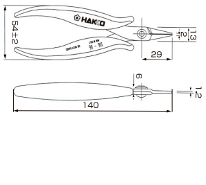
Part No. 106-06
