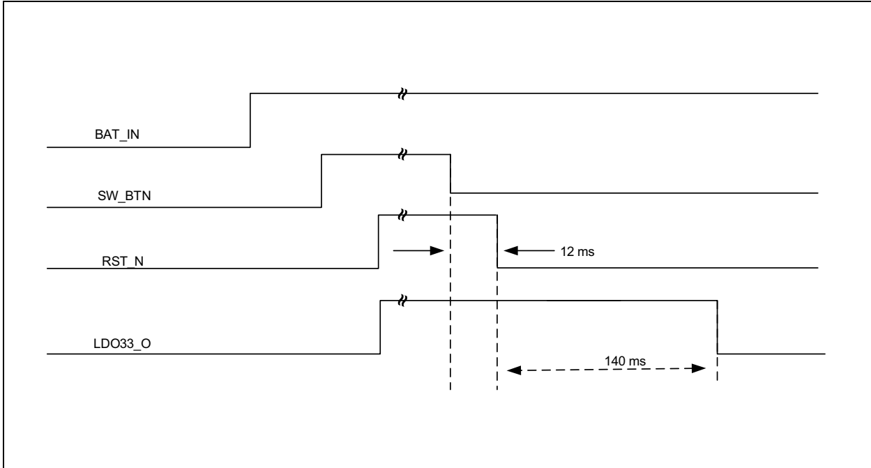
FIGURE 2-3: SW_BTN TIME (LOW) AT ACCESS STATES (1)
