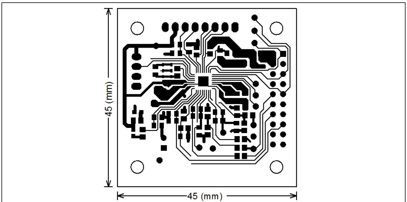
Figure 16 Top layer routing of the EVAL-M1-183M
