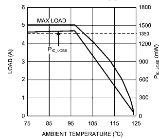
Current Derating ( V_{OUT} = 3.3\text{V} )
