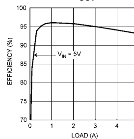
Efficiency ( V_{OUT} = 3.3\text{V} )
