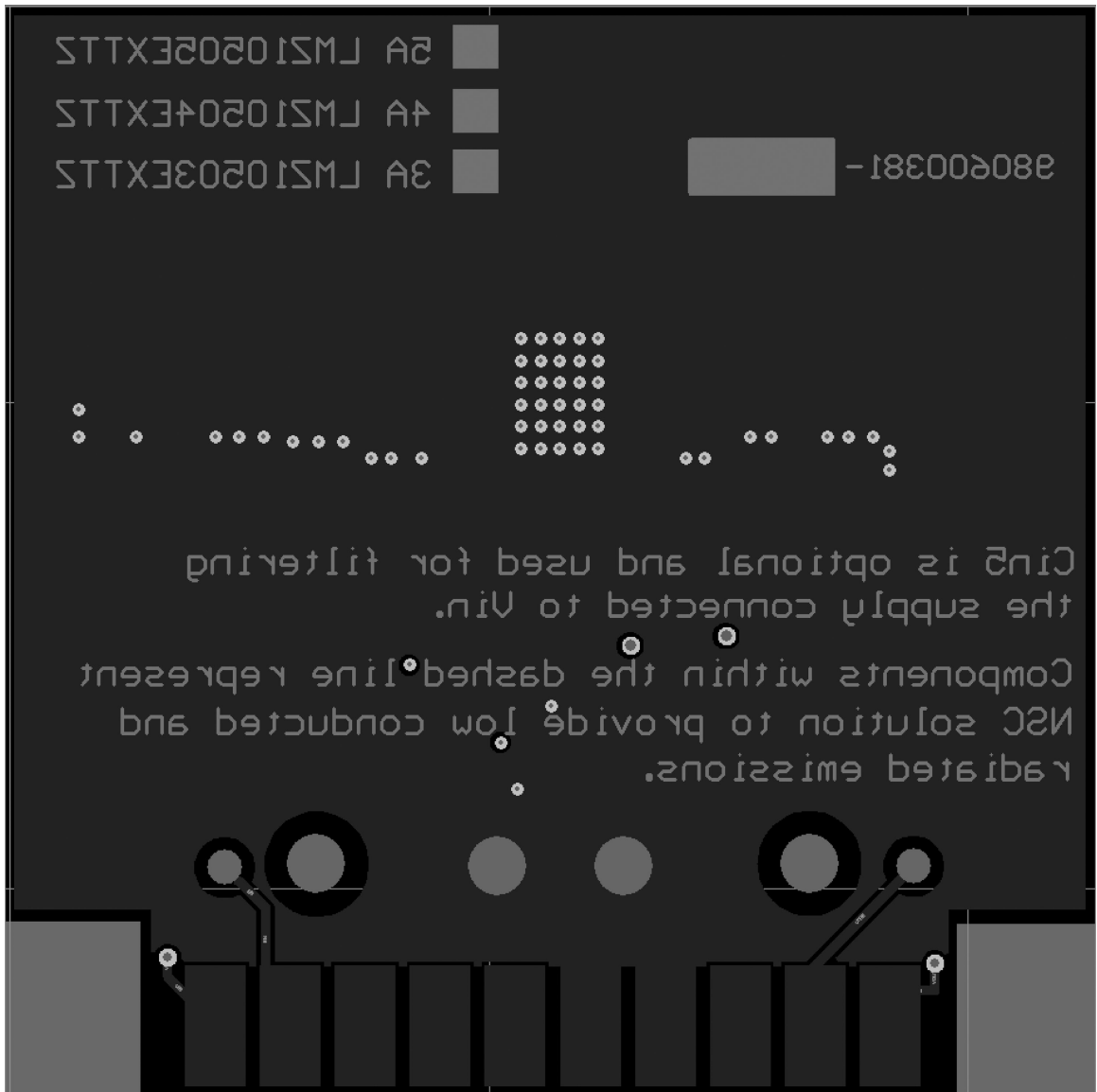
FIGURE 9. Bottom Copper
