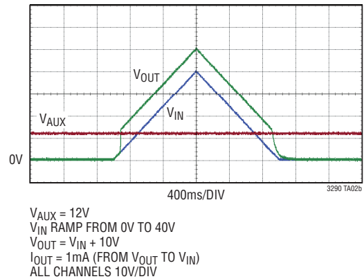
Figure 10. (V IN + 10V) Tracking Power Supply
