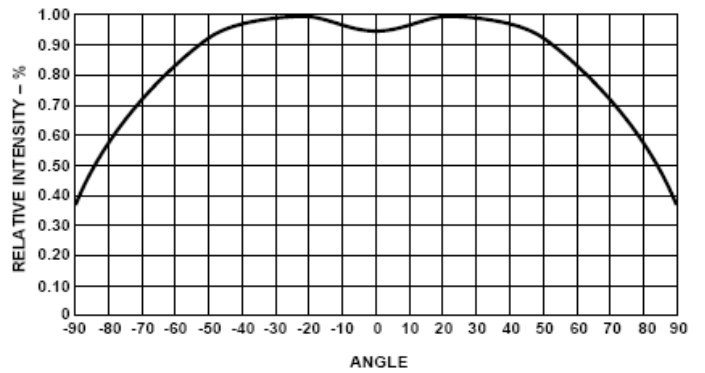
Figure 5: Radiation Pattern
