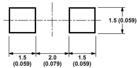
Figure 7: Recommended Soldering Land Pattern
