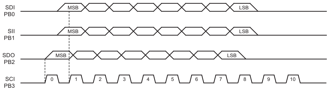
Figure 20-6. High-voltage Serial Programming Waveforms
