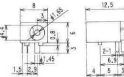
No.MJ-15 (5.5 φ × 2.5 φ mm)
