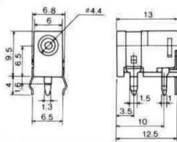
No.MJ-10 (center pin : 2 φ mm) Net Weight: 3 gr
