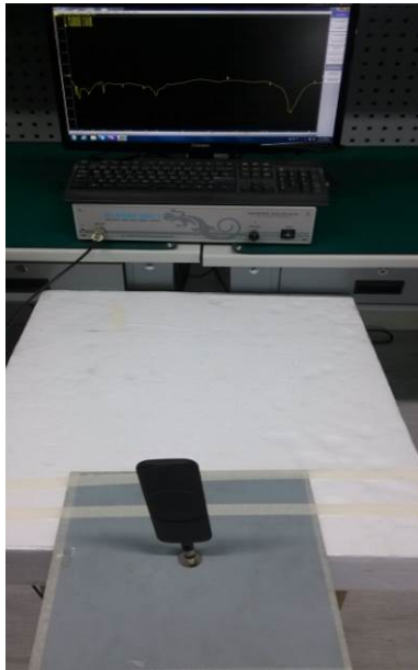
Antenna straight
