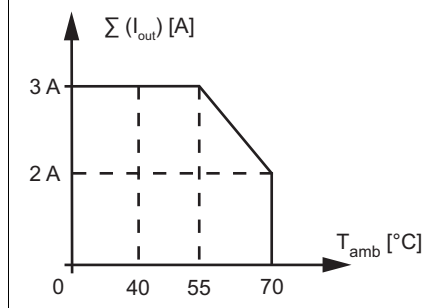
(2) BWU2594, BWU2713, Derating total current of outputs
