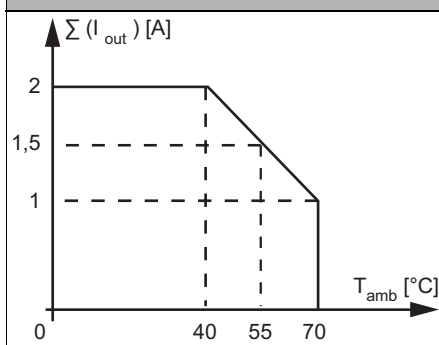
(3) BWU3141, BWU3539, BWU3456 Derating total current of outputs
