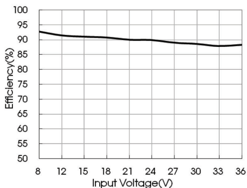
P7805-2000-S Efficiency Curve Efficiency vs. Input Voltage (at full load)
