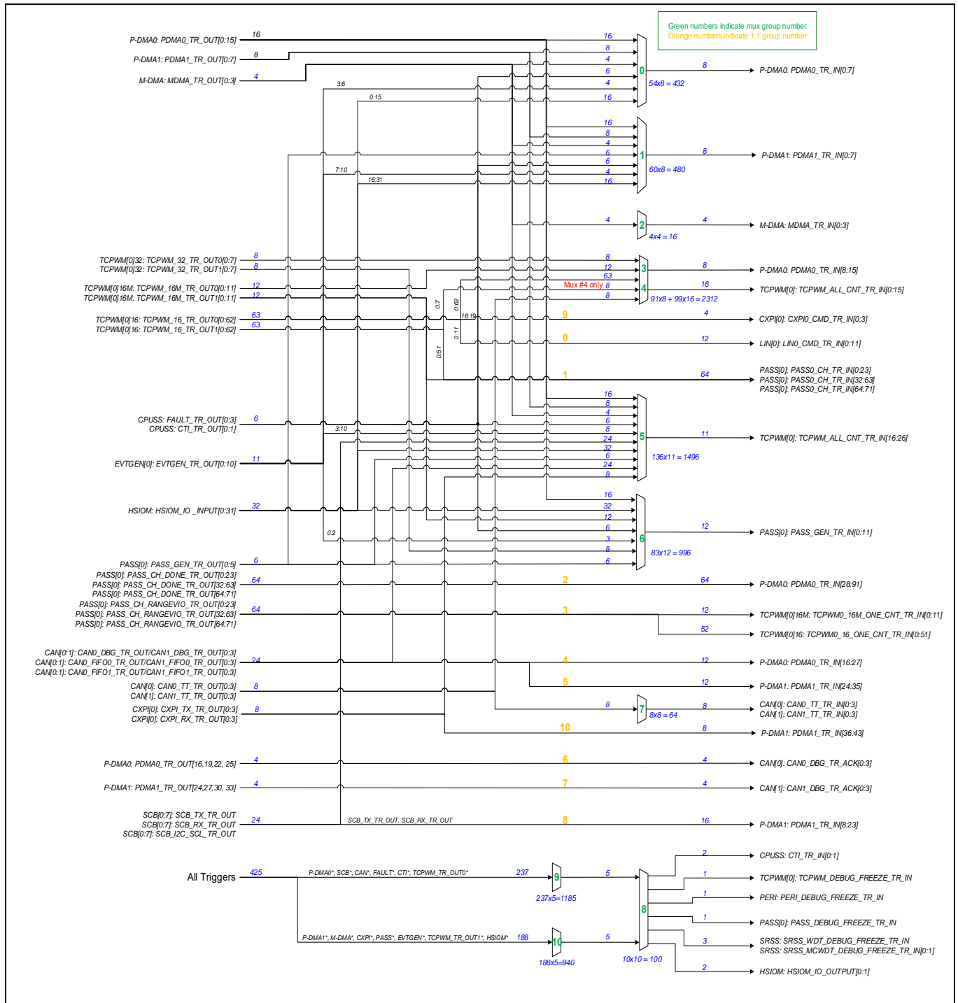
Figure 16-1 Trigger multiplexer [31]
