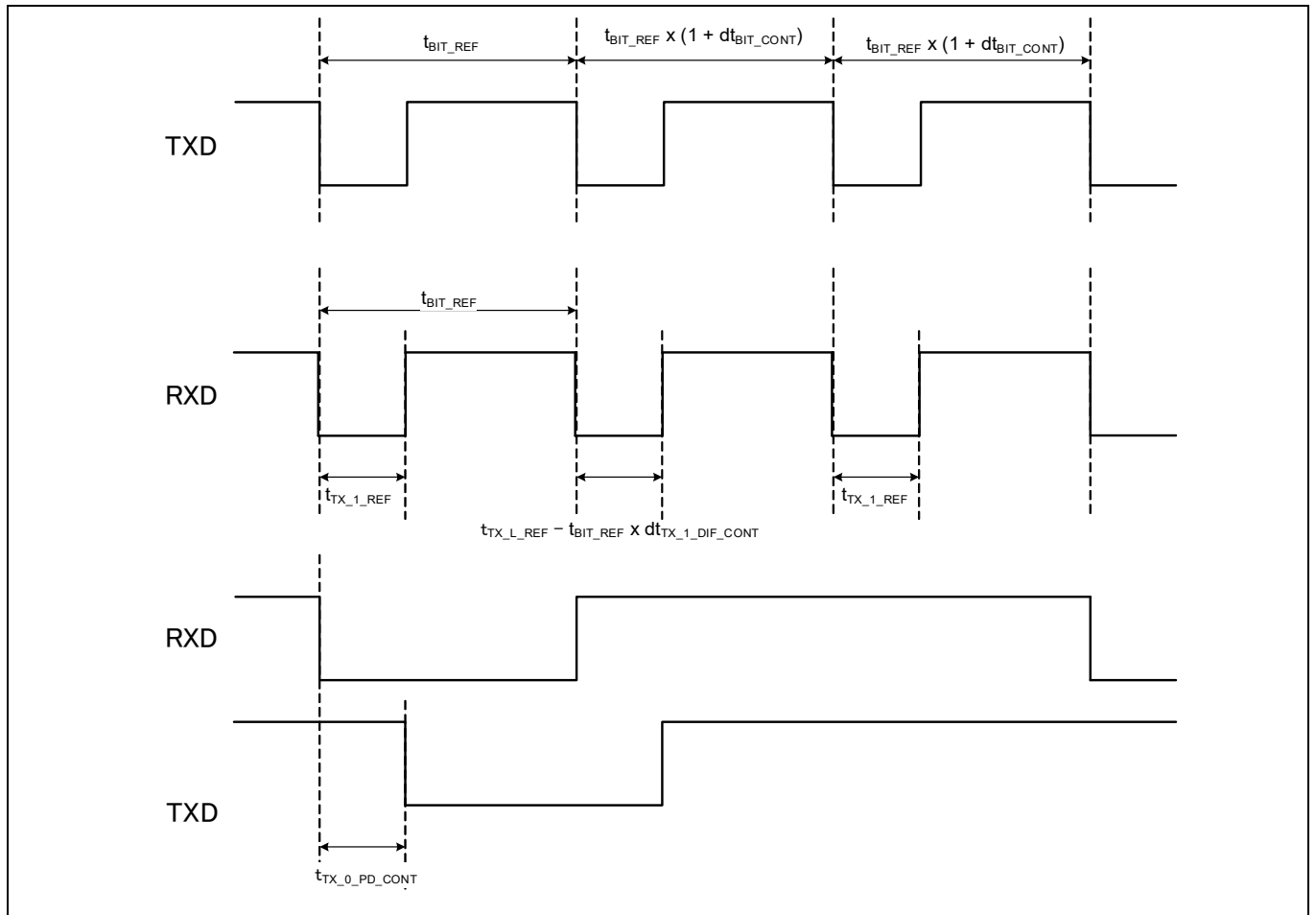
Figure 27-14 CXPI specifications
