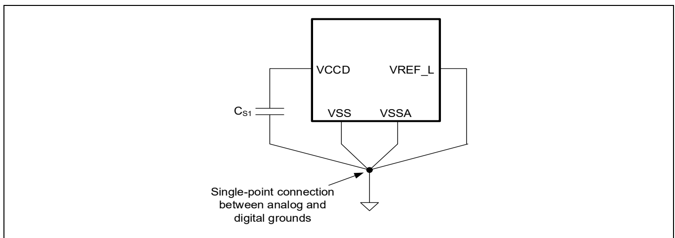
Figure 26-2 Smoothing capacitor
