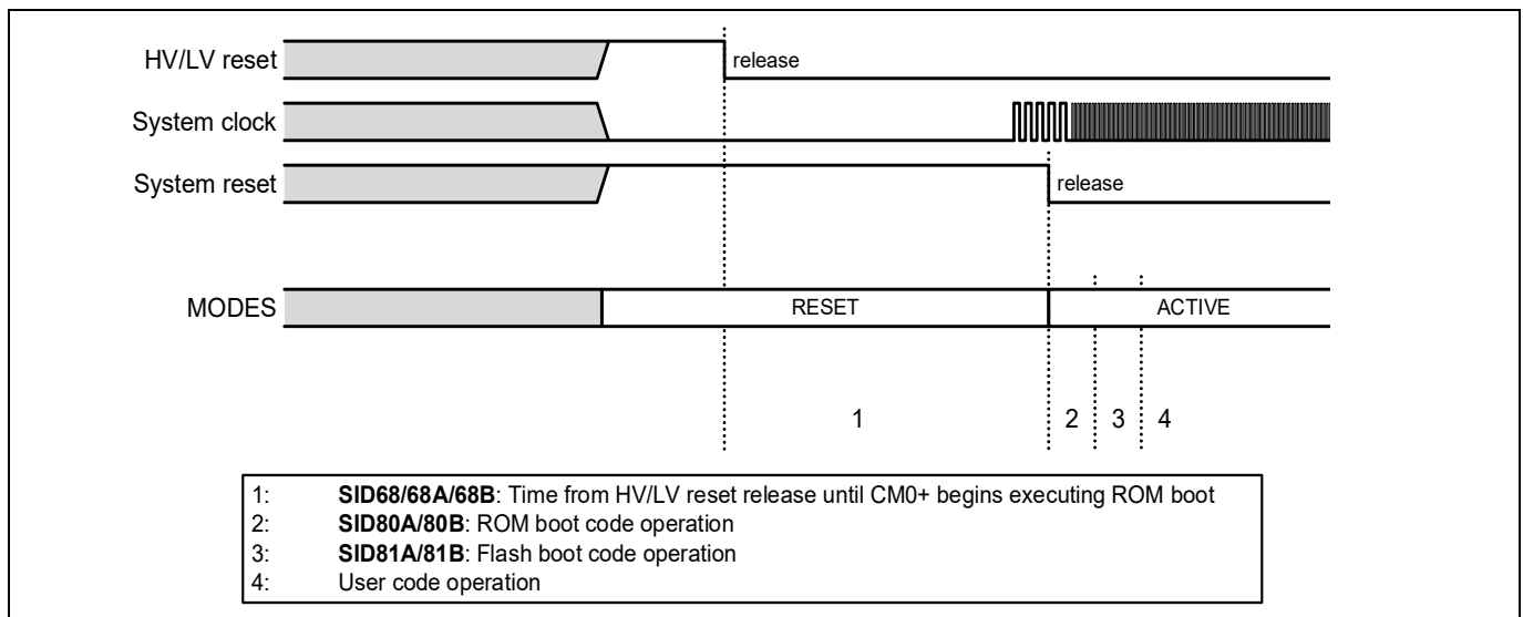
Figure 27-1 Reset sequence
