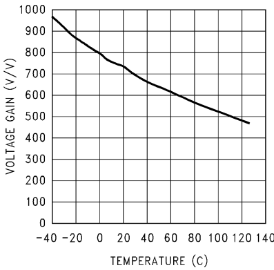
Error Amp Voltage Gain vs Temperature
