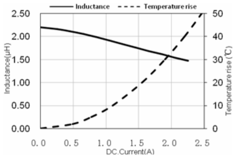
ASPI-U201610-2R2
