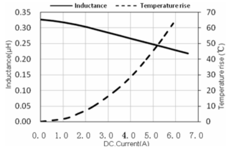
ASPI-U201610-R33
