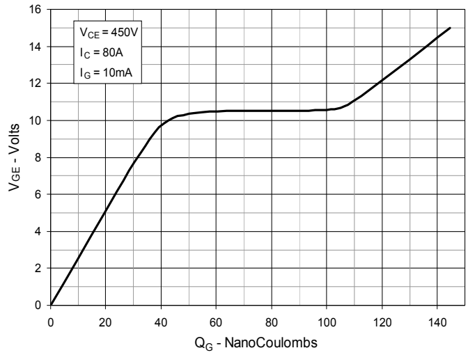
Fig. 8. Gate Charge
