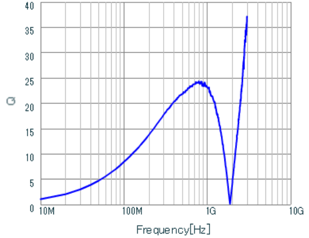
LQP03HQ68NJ02 Q.
