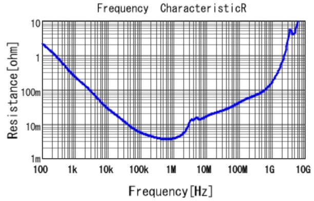
■ GRT31CC8YA106KE01 R DC0V, 25degC
