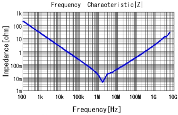
■ GRT31CC8YA106KE01 |Z| DC0V, 25degC
