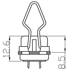
CENTRONIC SOLDER FEMALE TYPE WITH SPRING LATCH
