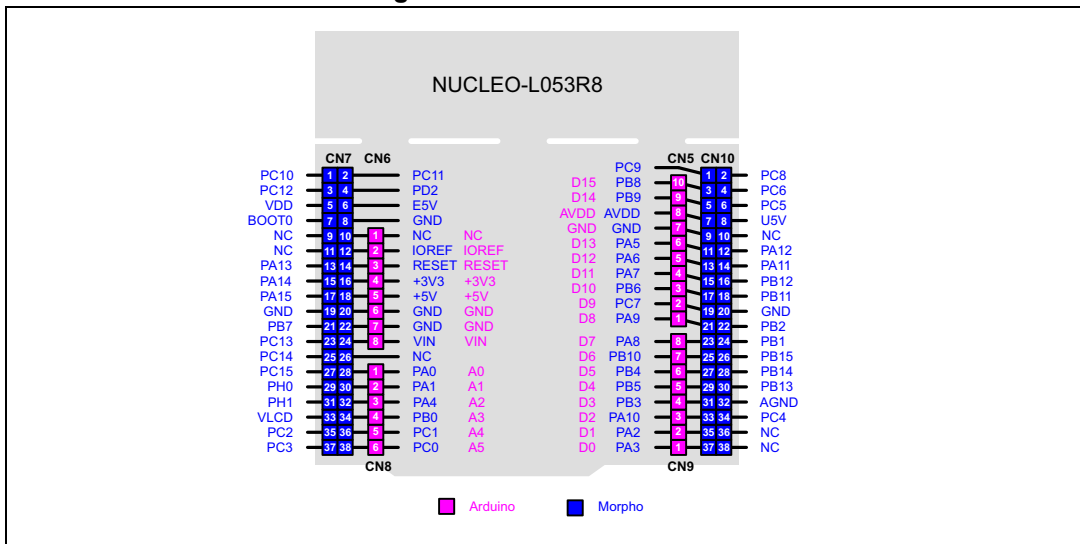
Figure 16. NUCLEO-L053R8
