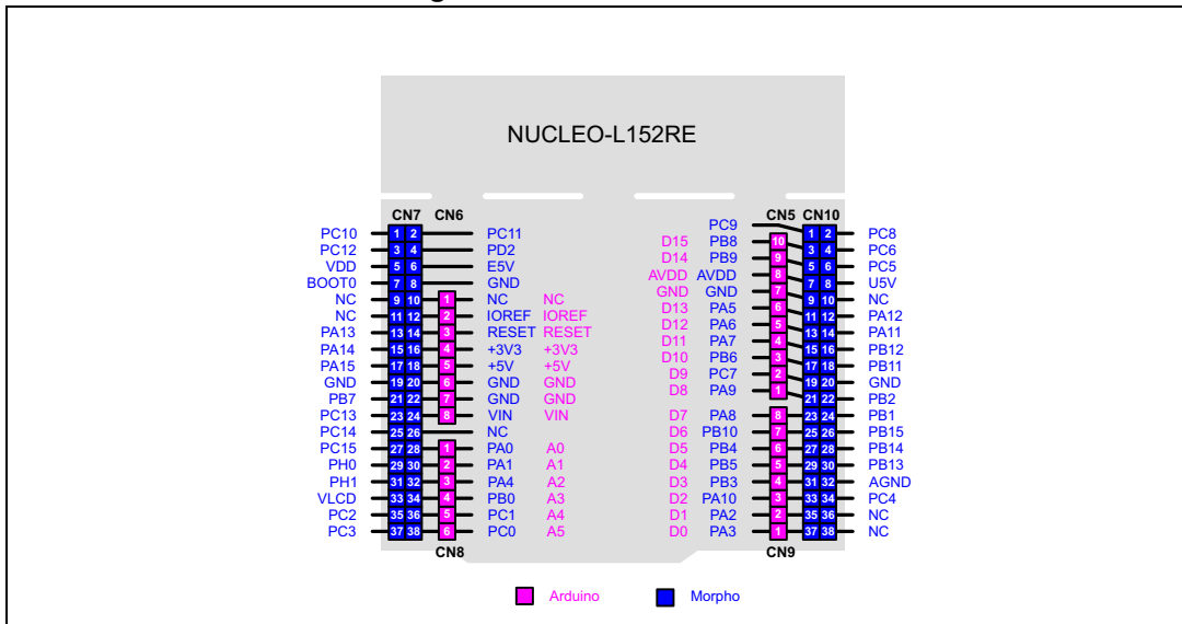
Figure 17. NUCLEO-L152RE
