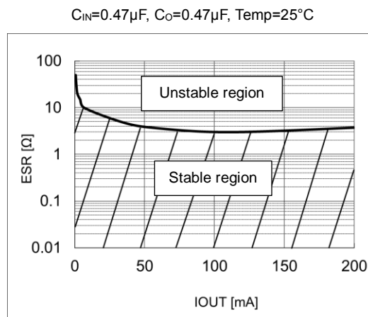
Figure 40. Stable region
