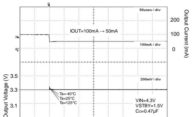
Figure 22. Load Response
