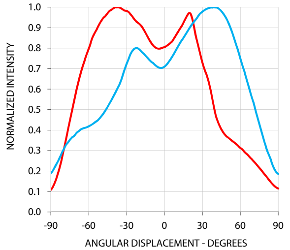
Figure 4. Radiation pattern
