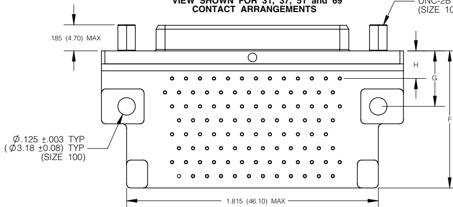
VIEW SHOWN FOR 100 CONTACT ARRANGEMENTS
