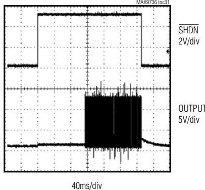
SHDN ON/OFF-RESPONSE
