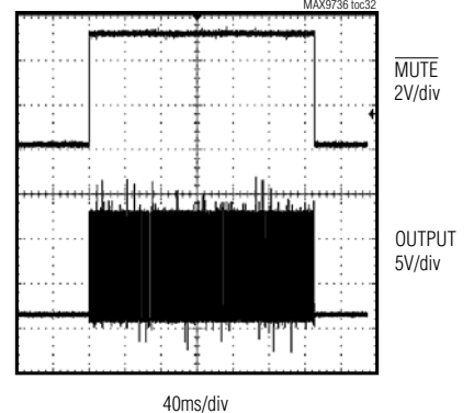
MUTE ON/OFF-RESPONSE
