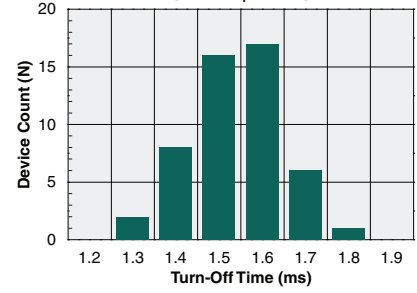
Typical Turn-Off Time (N=50, I F =5mA)
