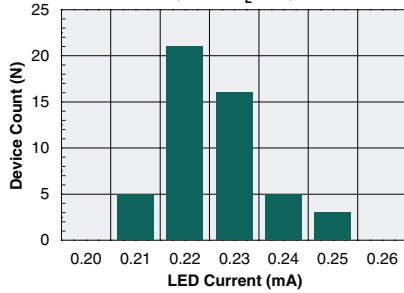
Typical I F for Switch Operation (N=50, I L =1A)
