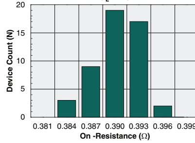
Typical On-Resistance Distribution (I L =1A)
