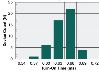
Typical Turn-On Time (N=50, I F =5mA)
