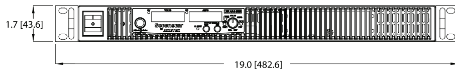
FRONT VIEW
