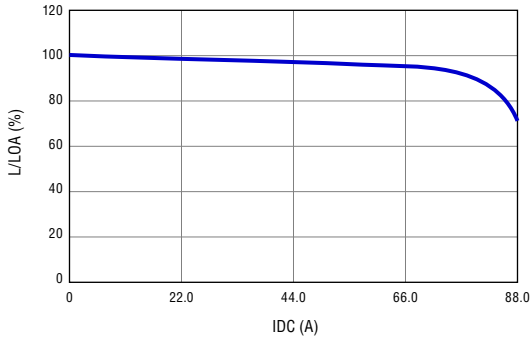
SPB1005-R12M
