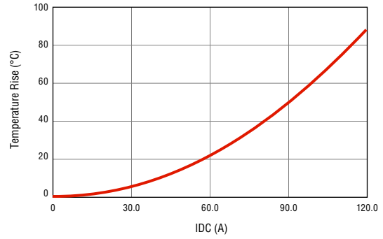
SPB1005-R12M
