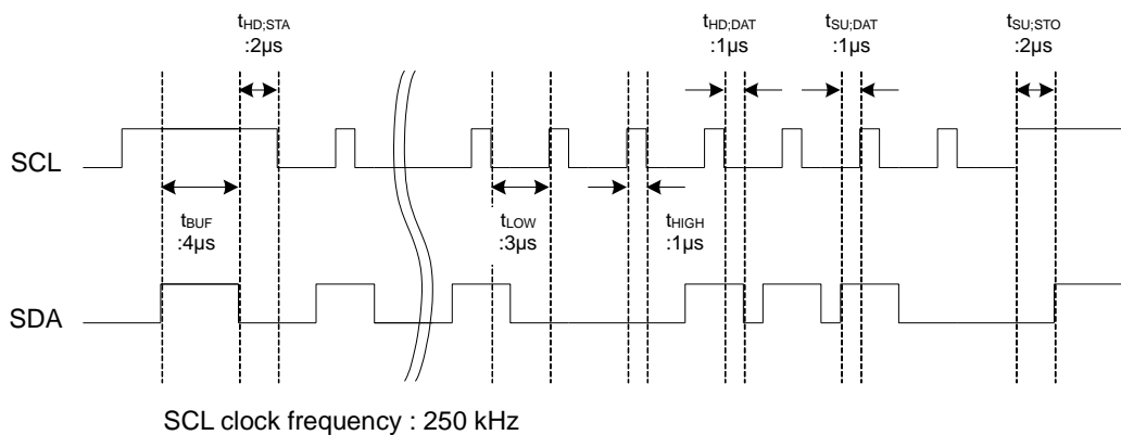
Figure 17. I 2 C Data Transmission Command Timing Diagram
