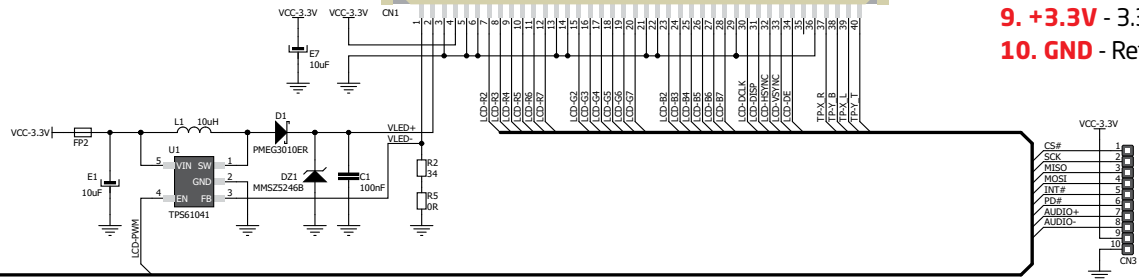
Figure 2: ConnectEVE schematic
