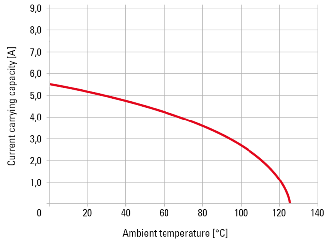
Current carrying capacity signal contact max. 5.1A at 20°C (4 of 80 pins)
