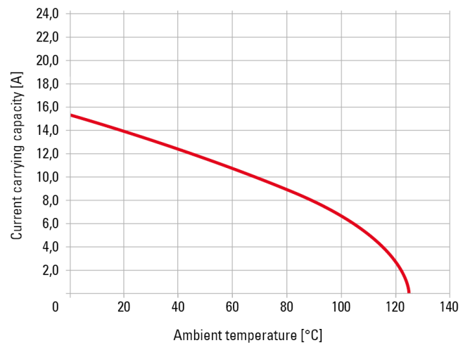
Current carrying capacity shield max. 14A at 20°C 80 pin, low-profile
