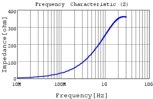
LQW18CN55NJ0H |Z|
