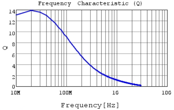
LQW18CN55NJ0H Q
