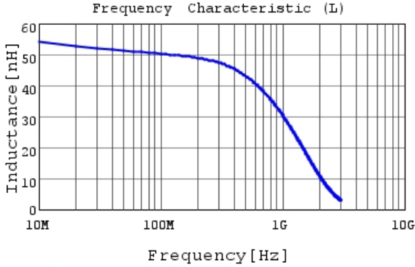
LQW18CN55NJ0H L
