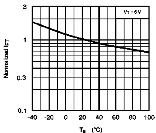
Fig. 12.6 Normalized I_T - T_a
