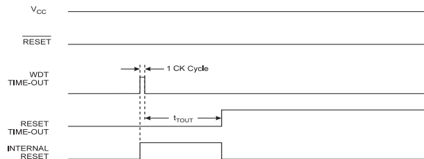
Figure 23-8. High-voltage Serial Programming Timing
