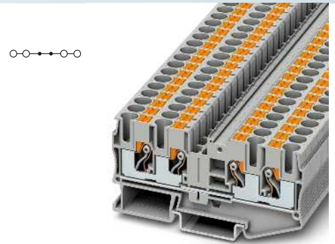
6 (10) mm 2 , 52 A, feed-through terminal block, 4 connections
